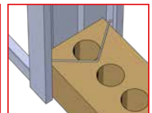
BRICK TIE
